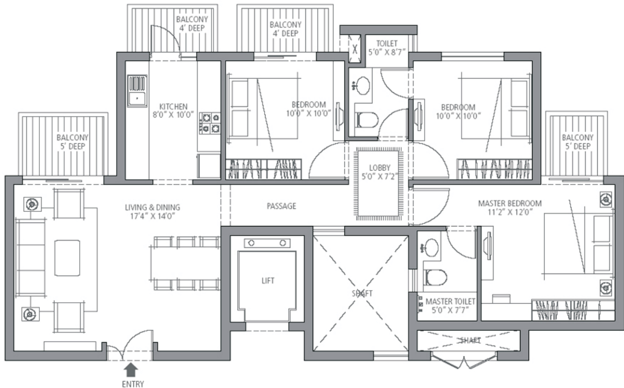
Key Plan - Towers A, B, C, D, F & G
